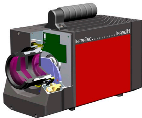
The motor focus unit is part of camera module 1 of the ImageIR®
